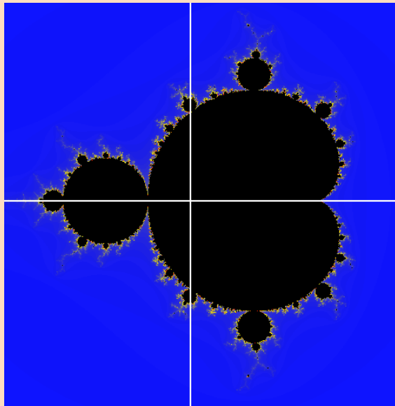
Mandelbrot Set
